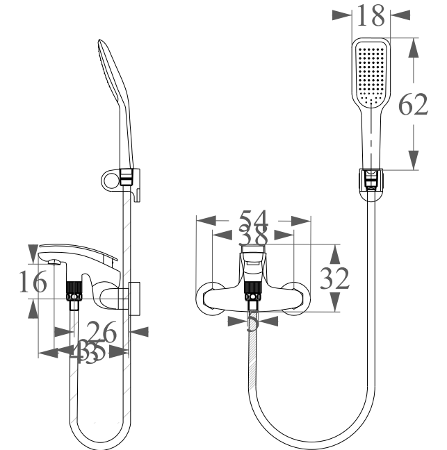
STALLONE Bath Shower Mixer System Chrome Cat. No. G1007773CH Sliding Handrail Chrome Cat. No. G7030701CH
