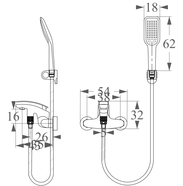
STALLONE Bath Shower Mixer System Red Cat. No. G1007773RD Sliding Handrail Chrome Cat. No. G7030701CH
