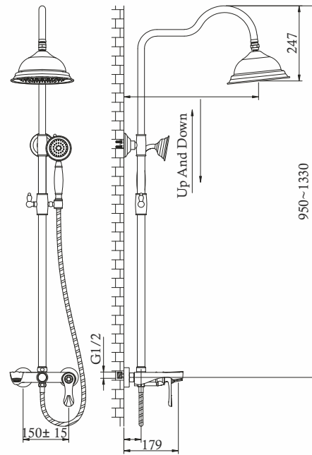
SAMANTHA Bath Shower Mixer System Jade Stone With Rose Gold Cat. No. G1001771JR
