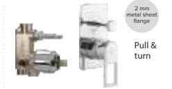
5 - Way (3 inlets + 2 outlets) single lever concealed diverter Exposed part without tipton & sleeve Concealed part with sleeve Exposed part #F1099712 Concealed part F4020101
