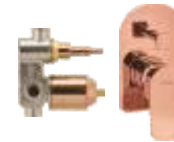
High flow single lever concealed diverter Exposed part without tipton & sleeve Concealed part with sleeve Exposed part #F1012721RG Concealed part #F4030101RG
