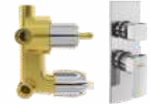
3 Outlet single lever concealed diverter Exposed part F1005731 Concealed part F4070202
